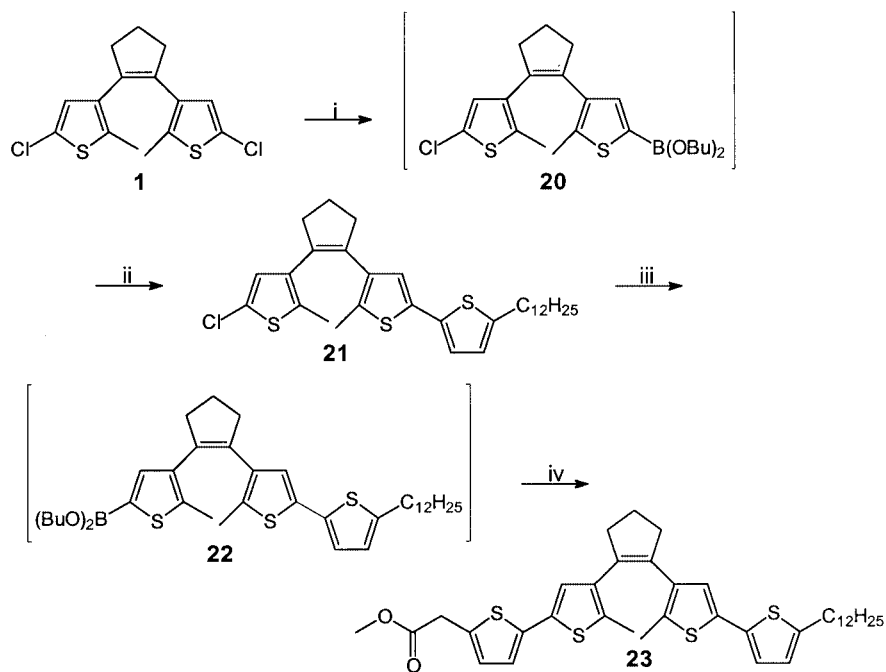
Scheme 7. Reagents: (i) n\text{BuLi} , room temperature, \text{B}(\text{O}i\text{Bu})_3 ; (ii) 2-bromo-5-dodecylthiophene, \text{Pd}(\text{PPh}_3)_4 , \text{Na}_2\text{CO}_3 , ethylene glycol, reflux, \text{H}_2\text{O} , THF, 37%; (iii) t\text{BuLi} , room temperature, \text{B}(\text{O}i\text{Bu})_3 ; (iv) methyl 2-(5-bromo-2-thienyl)acetic acid, \text{Pd}(\text{PPh}_3)_4 , \text{Na}_2\text{CO}_3 , ethylene glycol, reflux, \text{H}_2\text{O} , THF, 32%
